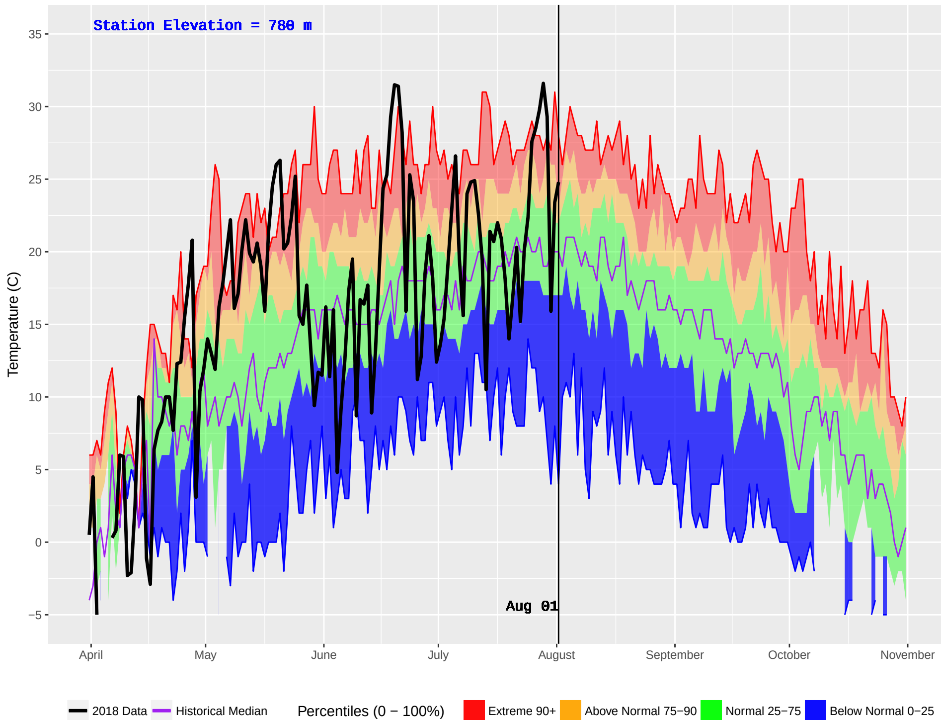
MUSKWA (131) : Historical (1983–2016) and Current (2018) Daily Temperature
