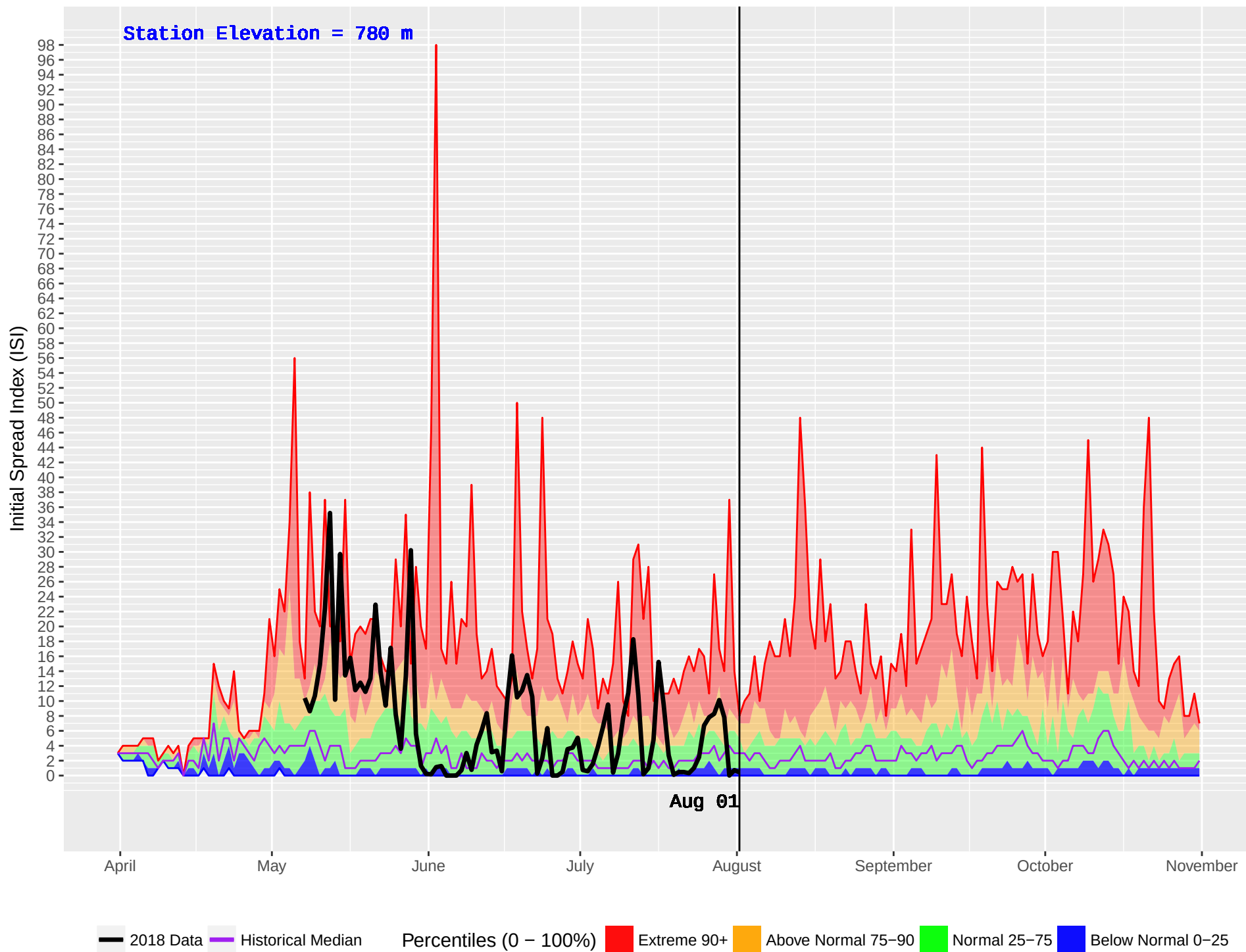
MUSKWA (131) : Historical (1983–2016) and Current (2018) Daily Initial Spread Index (ISI)
