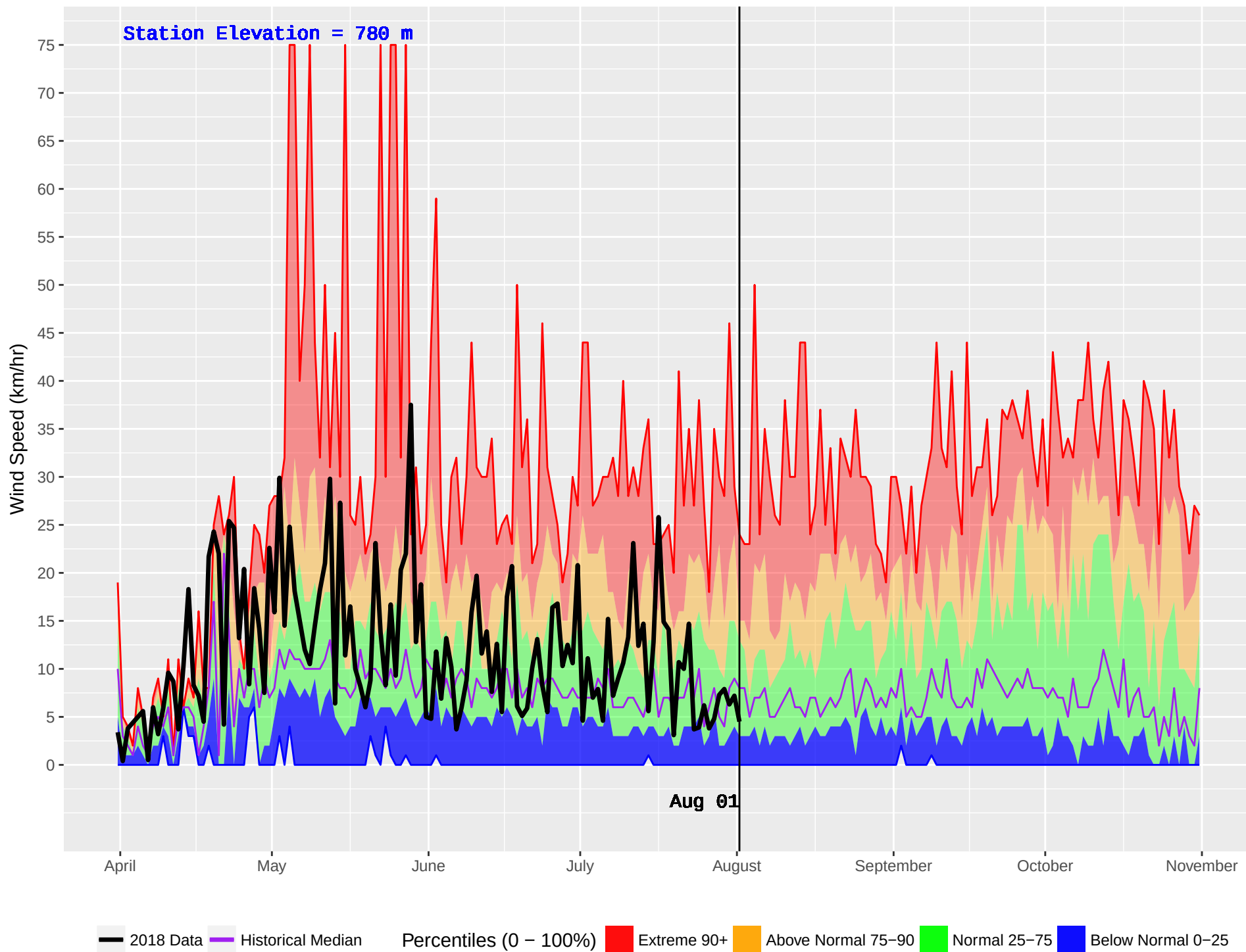
MUSKWA (131) : Historical (1983–2016) and Current (2018) Daily Wind Speed
