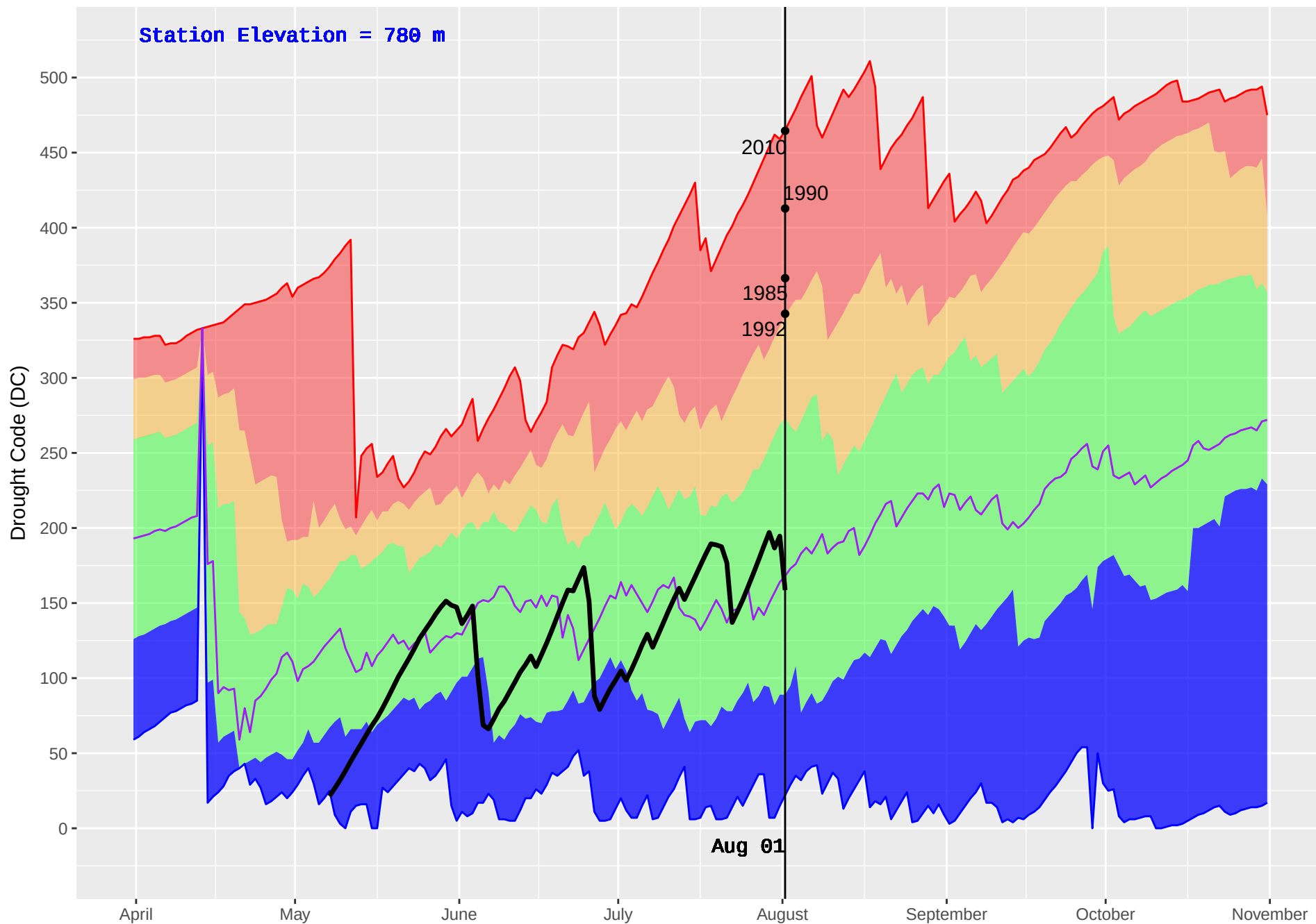
MUSKWA (131) : Historical (1983–2016) and Current (2018) Daily Drought Code (DC)
