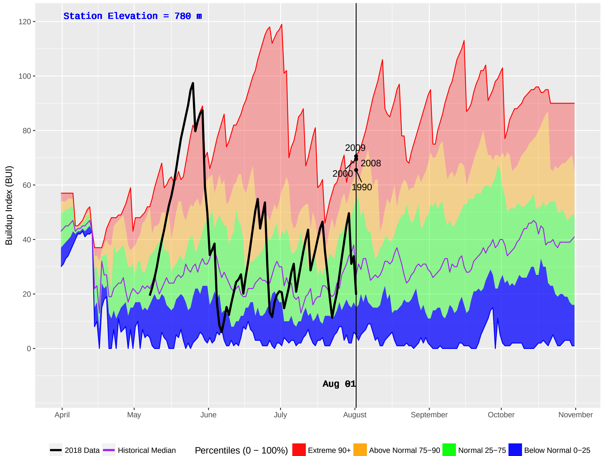
MUSKWA (131) : Historical (1983–2016) and Current (2018) Daily Buildup Index (BUI)
